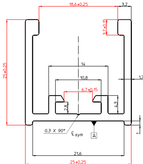
HK3106: U-profile
